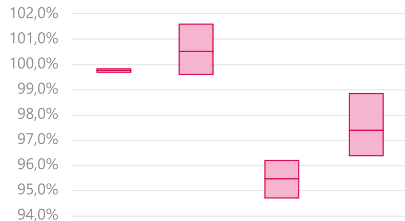
Figure 6: Impact GLOSA on green wave corridor
